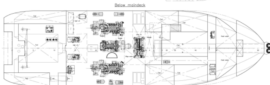
Below maindeck
