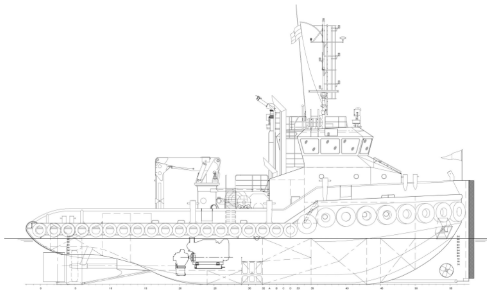
Forecastledeck
